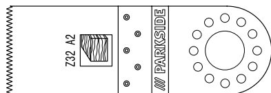
Plunge saw blade (32mm) Z32 A2 [6]
