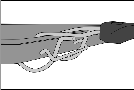
Fig. 2: Hooking the tongs 10 onto the baking tray 9
